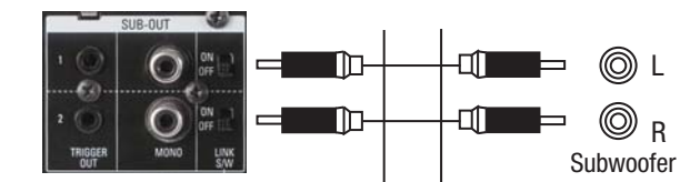
Figure 3 – Subwoofer
