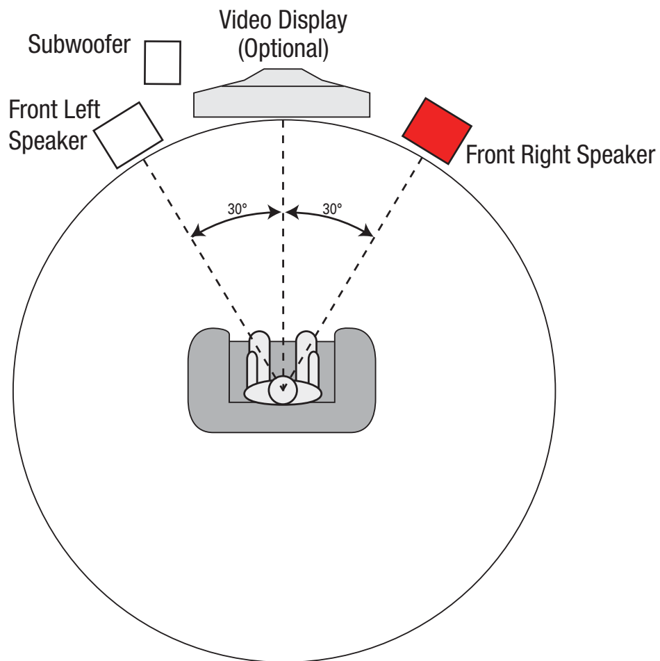
Figure 10 – Speaker Placement
