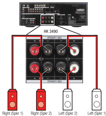
Figure 11 – Speaker Connections
