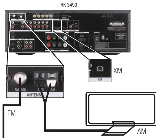
Figure 13 – Antenna Connections
