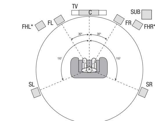
Speaker Positioning for 7.1-Channel Systems (AVR 1710S/AVR 171S only) (Middle: with Surround Back Speakers; Bottom: with Front Height Speakers)
